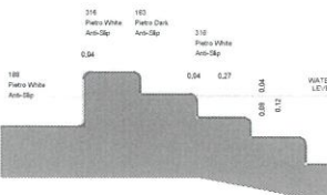
FOOTBATH AND STAIRS DETAIL A1 SC 1/10 A3 SC 1/20
