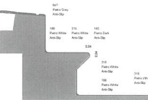
SEAT DETAIL A1 SC 1/10 A3 SC 1/20
